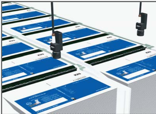
Two optical character recognition MVS cameras are set-up to verify the proper page order before binding catalog.
